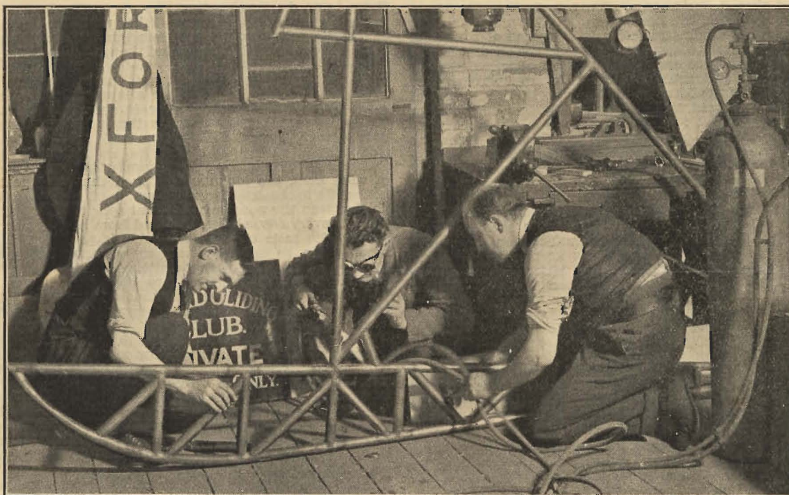
The welded steel-tube fuselage of the primary machine which the Oxford Gliding Club are building. This is so far as we know the first welded glider yet built in this country. "THE SAILPLANE" suggests that from the photograph the junction between the skid and the king-post appears inadequate. Also the diagonal bracing struts are offset as is NOT done in aircraft.
