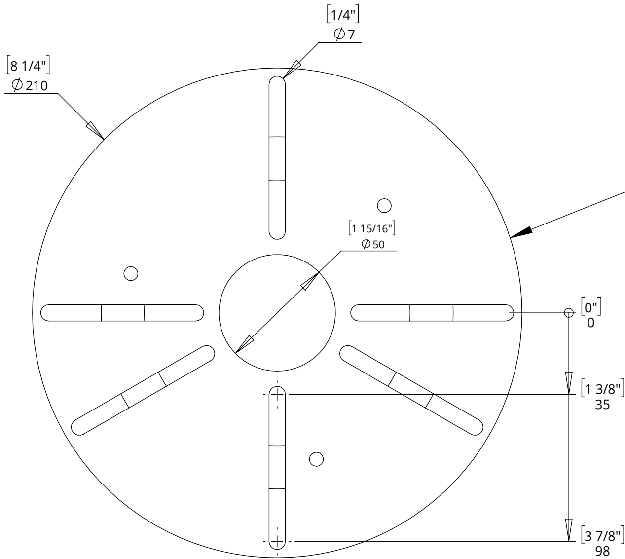
Camera Mount Plate
