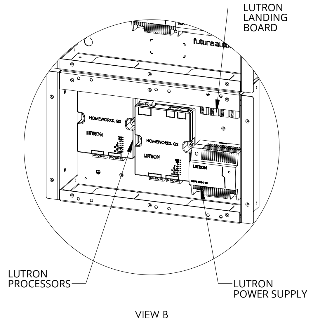
LCP PDPS - POWER SUPPLY ADD ON UNIT (NOT SUPPLIED)
