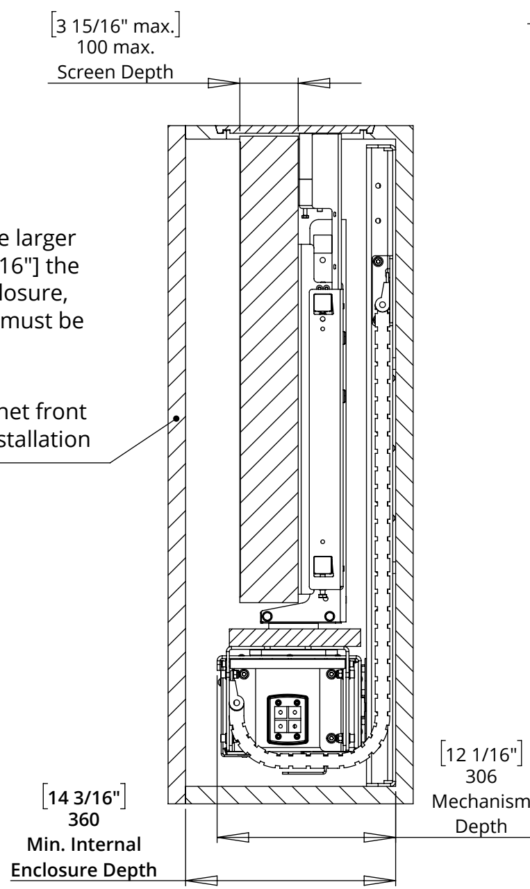
SECTION A-A MECH DOWN
