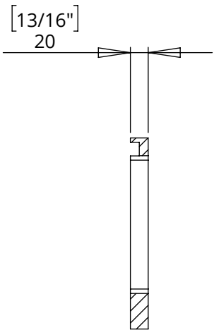
SECTION G-G
