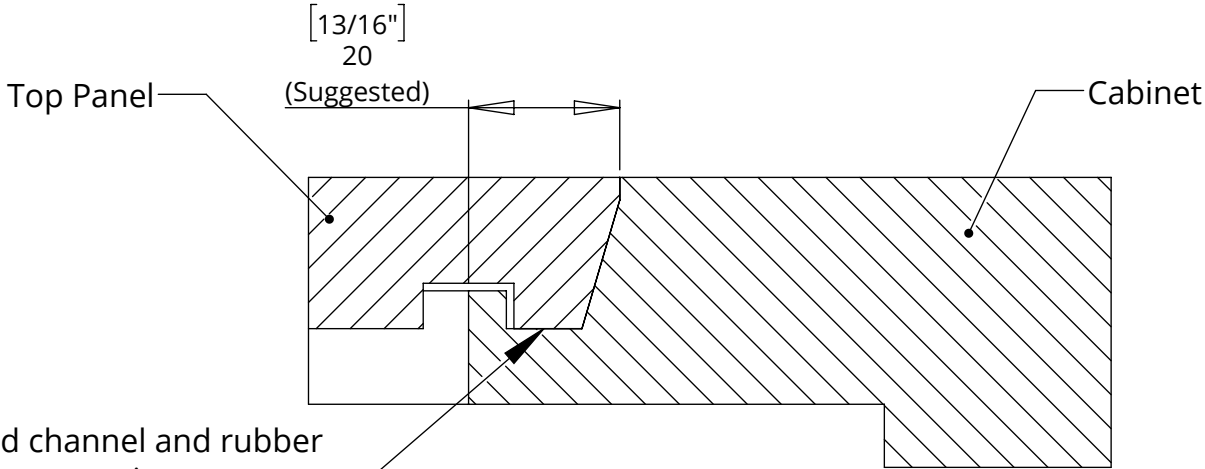
DETAIL B
