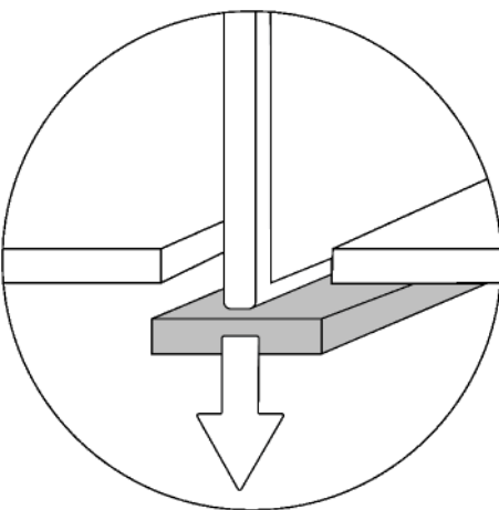
I - INVERTED See I-LSH-MO Tech
