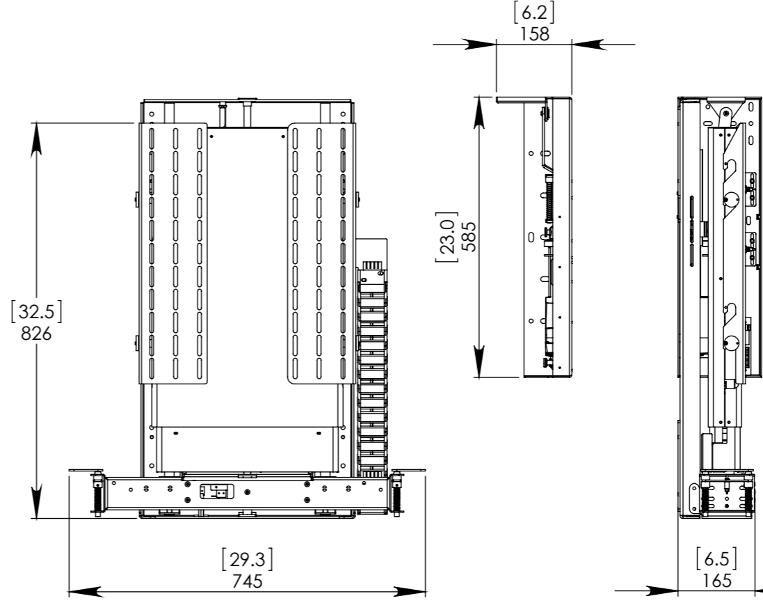
MECHANISM - DOWN POSITION
