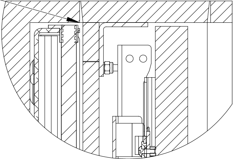
DETAIL F
