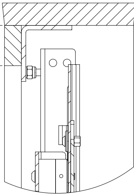
DETAIL Q
