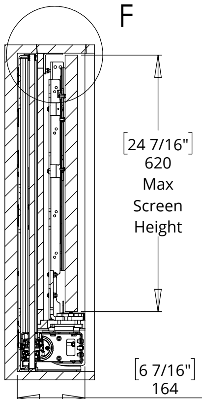
SECTION E-E
