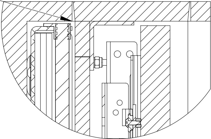
DETAIL F
