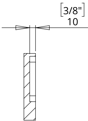
SECTION G-G
