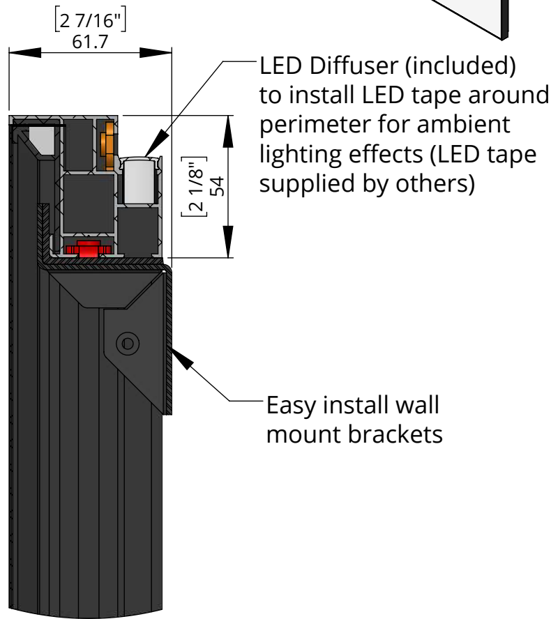
DETAIL BB SCALE 1 : 2
