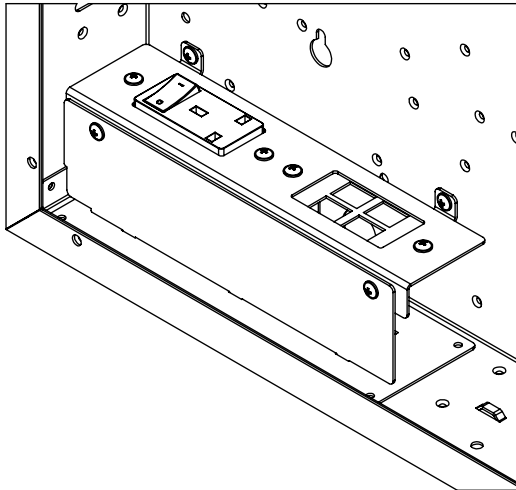
SWITCHED MPO AND KEYSTONE
