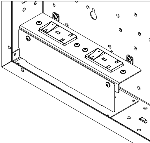
DUAL MPO OUTLETS
