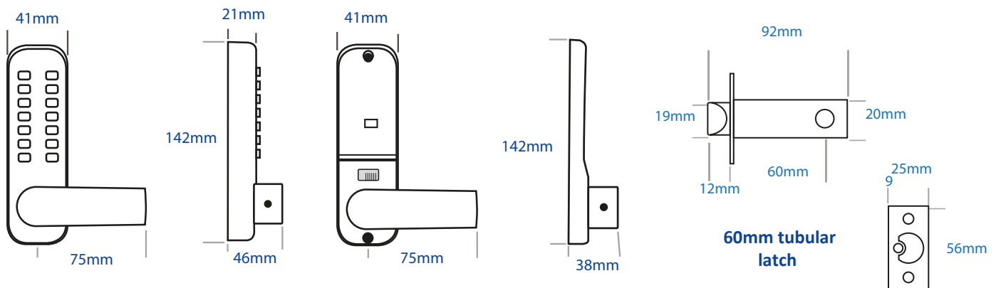
2400 Series Inside Handle
