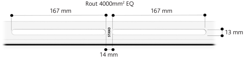
Internal Vent
