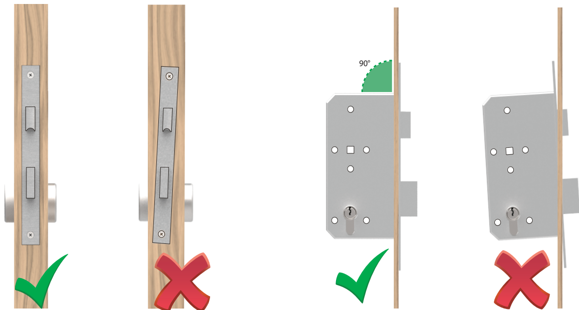
Figure 2 - Correct installation of a lockset
