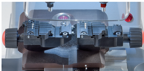
Tilting clamps (0° +/- 45°) with 3 seats of key positioning
