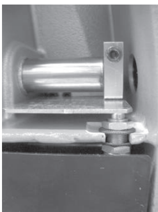
Fig. 62 - micro-switch OFF
