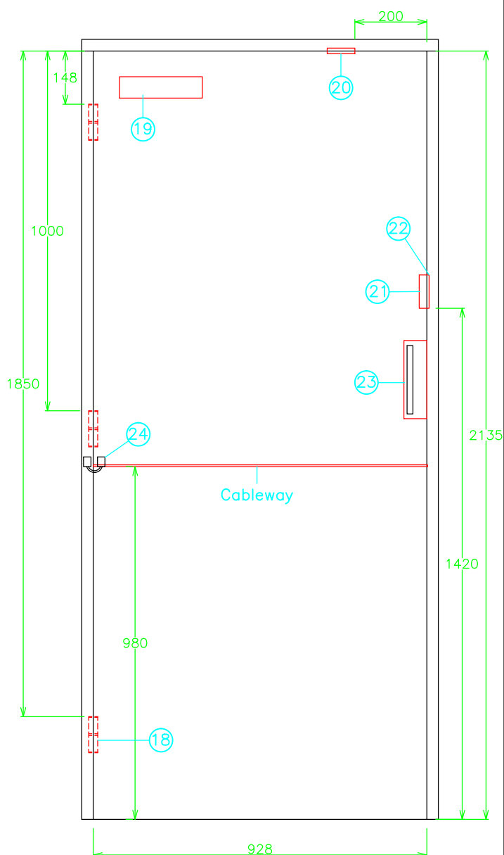
Doorset B
