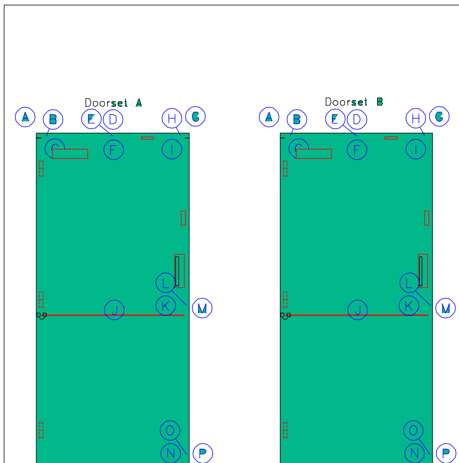
Doorset A - (leaf hung on the left and opening in towards the furnace)
