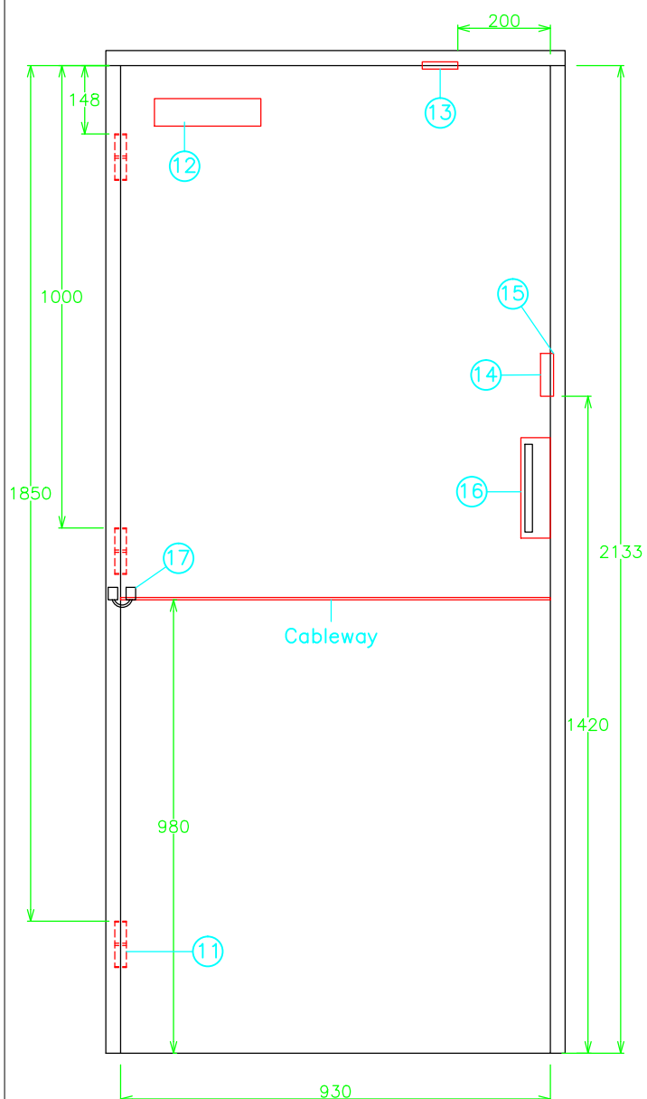
Doorset A
