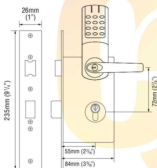
CL5020 NetCode® Mortice Lock
