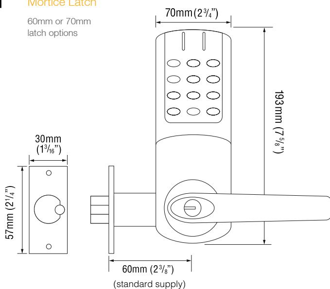
CL5010 NetCode® Mortice Latch
