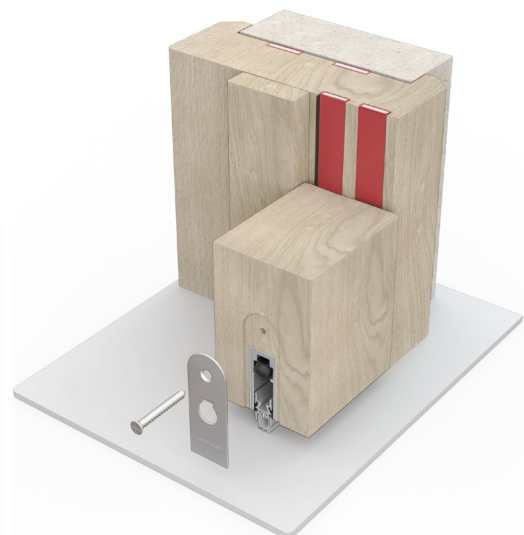
FD60 example: AS seal (Shown with LP1504 fire seal & LAS8001 si + cladding kit)
