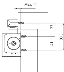
2320B.T Door mount pull side Max. opening angle 180°
