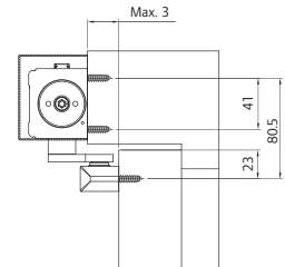
2321B.T Transom mount pull side Max. opening angle 180°
