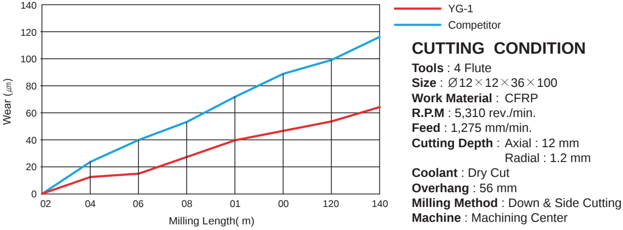
YG-1 (Total Milling Length 140m)
