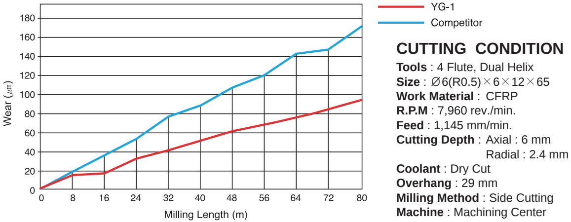
YG-1 (Total Milling Length 80m)
