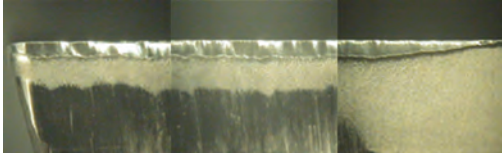
Competitor A (Total Milling Length 140m)
