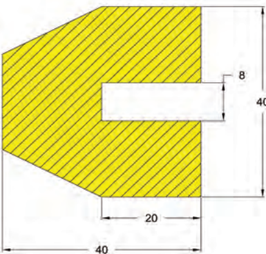
Trapeze 40 x 40 x 8
