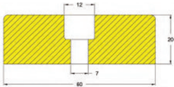
Rectangle 60 x 20, 3 pre-drilled holes
