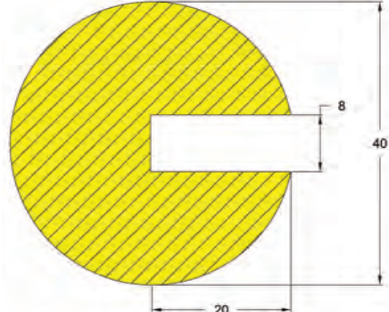
Semi Circular 40 x 40 x 8
