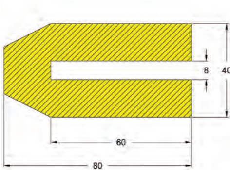
Trapeze 40 x 80 x 8
