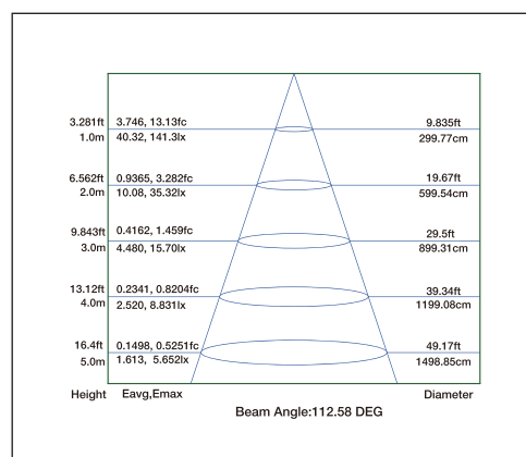
Illuminance-Distance Curve
