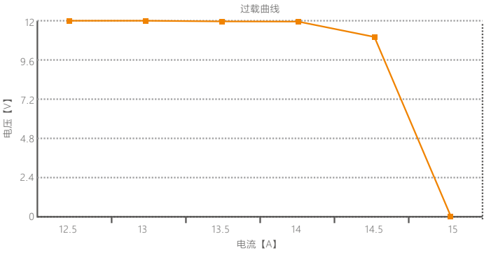
LM-150-12-G1D2
