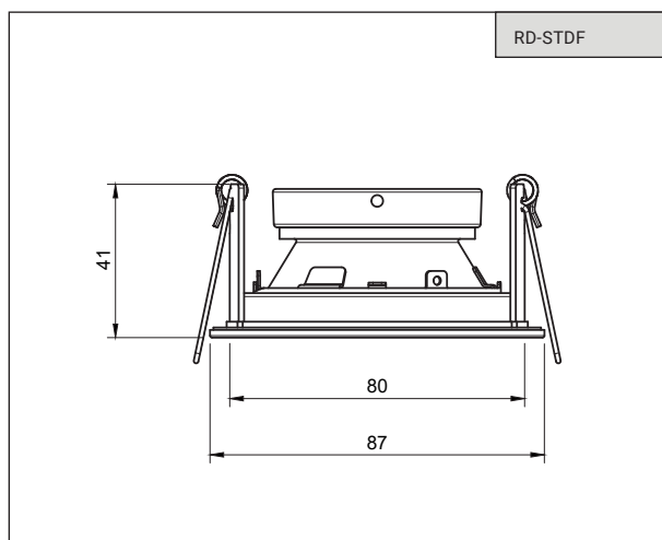
Standard Fixed Recessed Downlight
