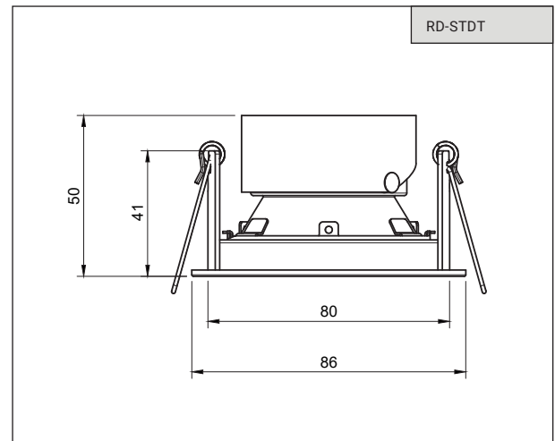
Standard Tilttable Recessed Downlight
