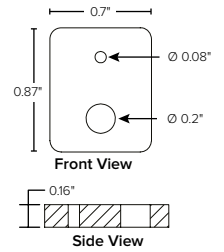
Hanger Block
