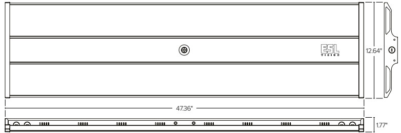
ESL-LHB-255400W-44050
