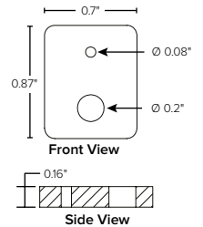
Hanger Block
