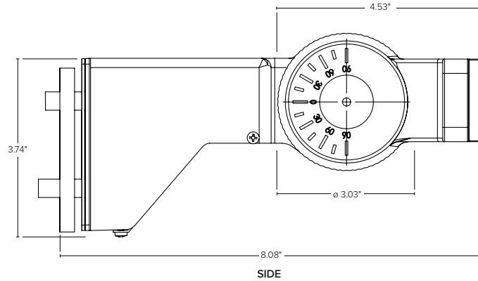
SIDE
