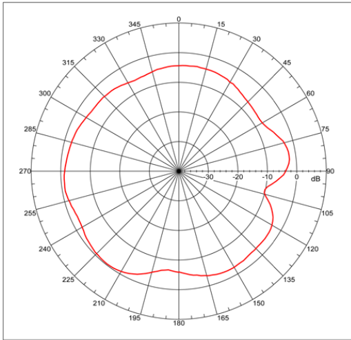
Far-Field Amplitude H-Plane
