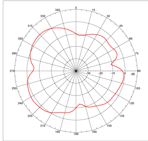
Far-Field Amplitude E-Plane
