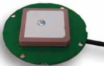
Figure 2: L1/L2 GPS with ceramic patch
