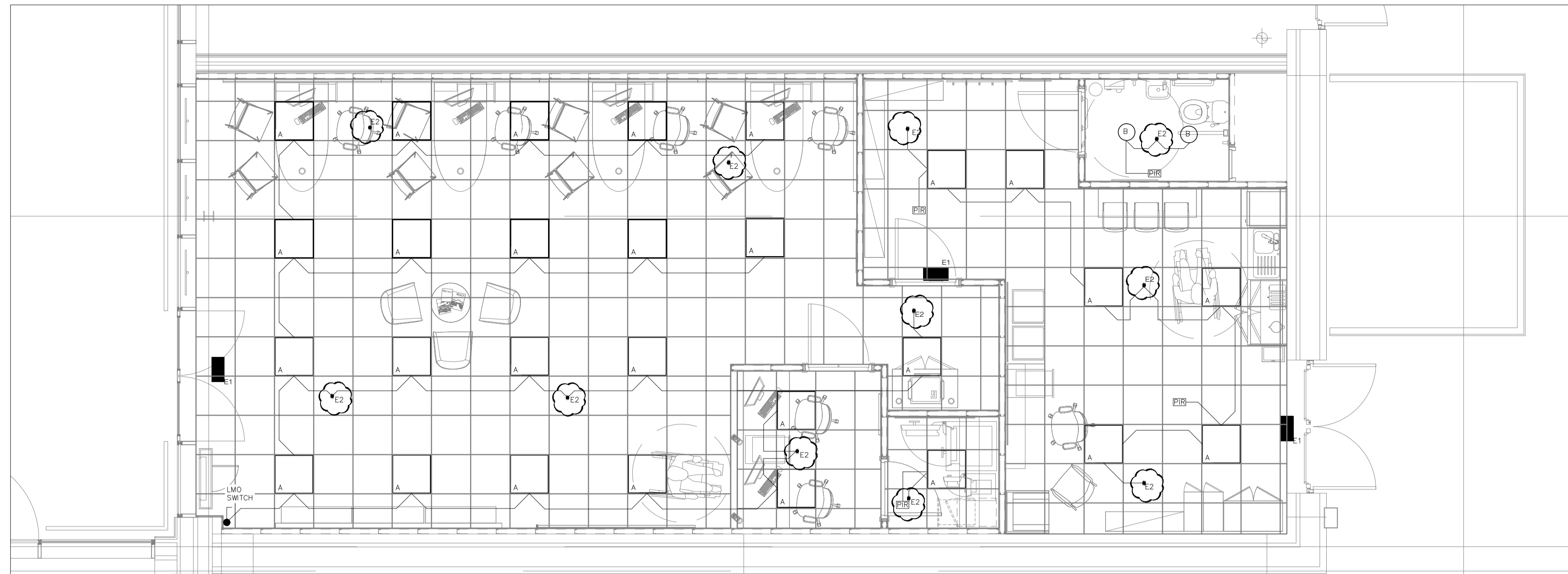
A GROUND FLOOR - LIGHTING PLAN E-101 SCALE - 1:50
