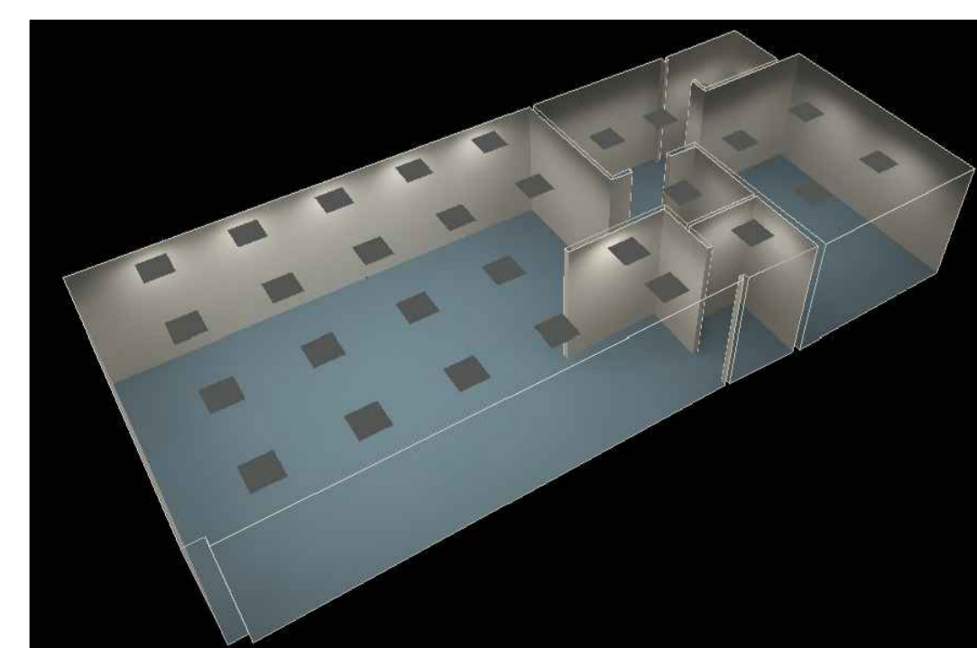
F LIGHTING LUX LEVELS - AXONOMETRIC VIEW E-101 SCALE - NTS
