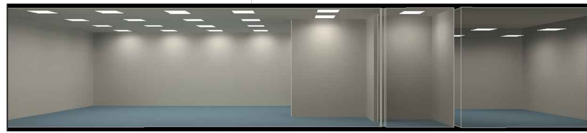
C LIGHTING LUX LEVELS - SECTION A-A E-101 SCALE - NTS
