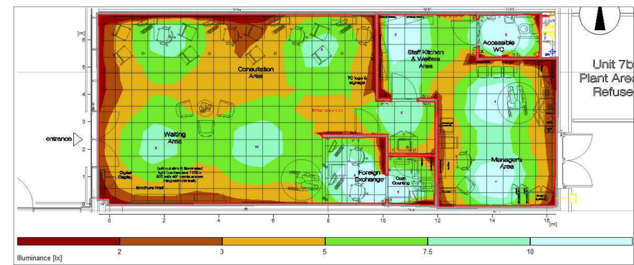
B EMERGENCY LIGHTING LUX LEVELS E-101 SCALE - NTS
