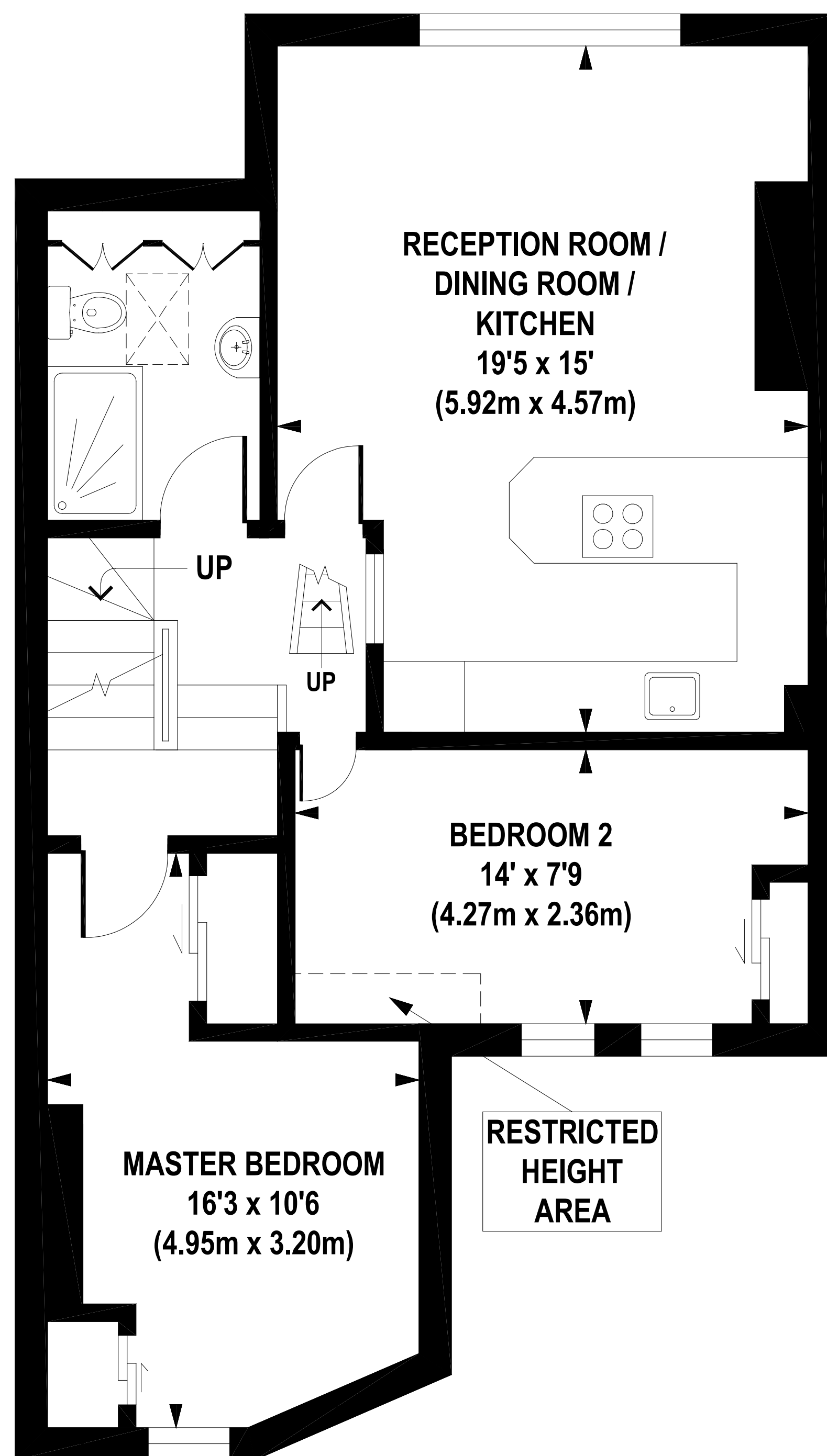
SECOND FLOOR GROSS INTERNAL FLOOR AREA 679 SQ FT
