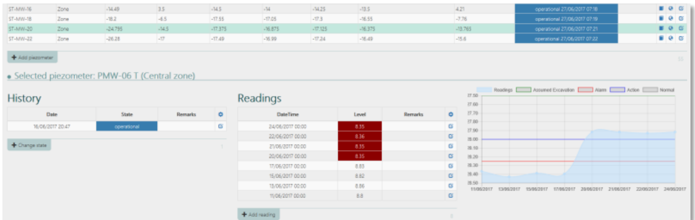
Piezometer management
