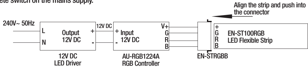
Diagram 1 - Connections
