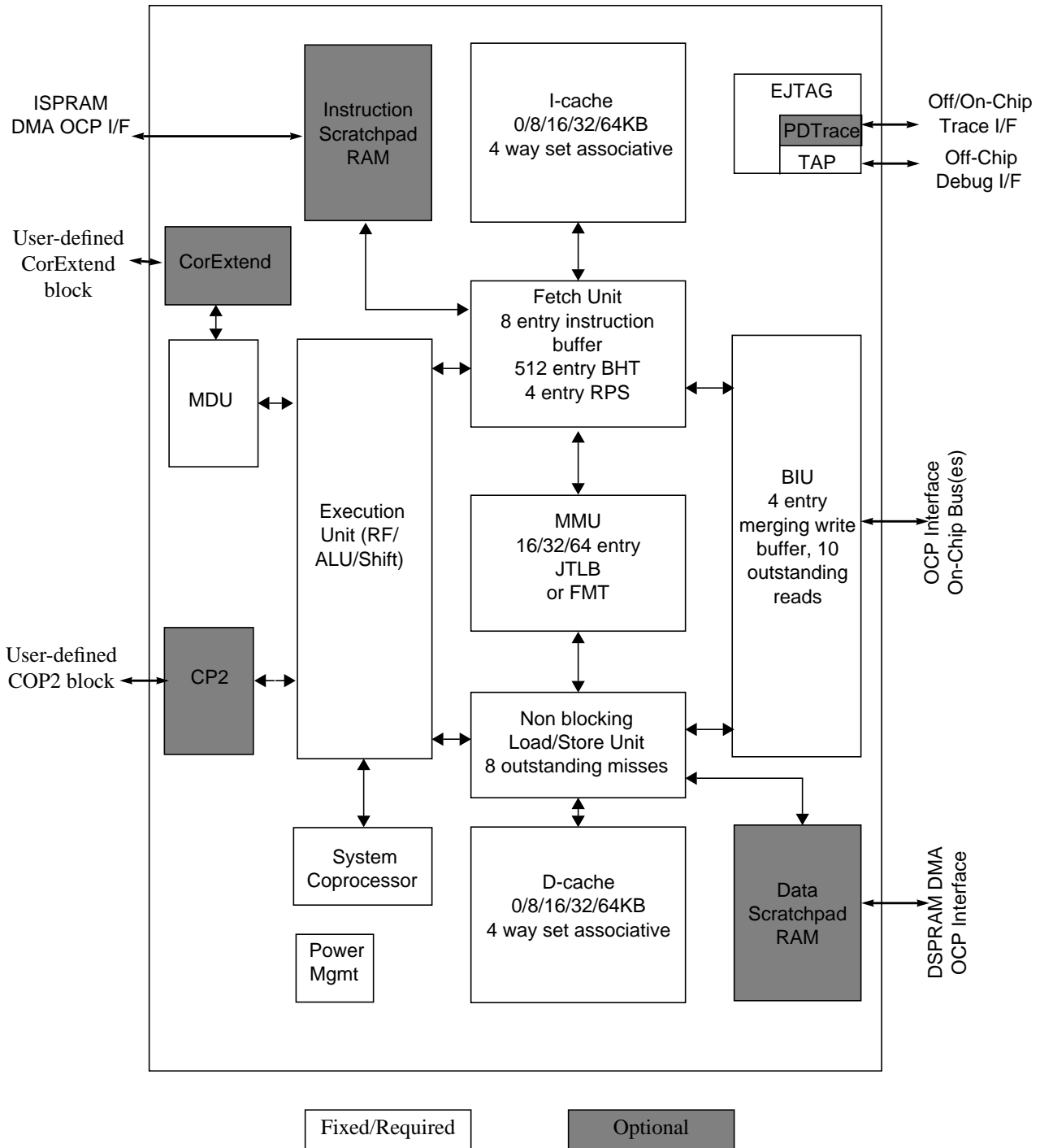
Figure 1 24Kc™ Core Block Diagram
