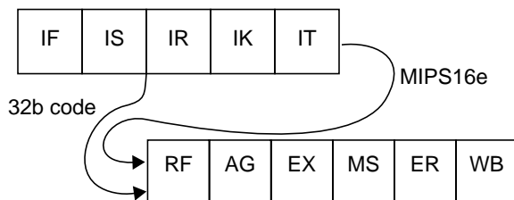
Figure 2 24Kc™ Core Pipeline
