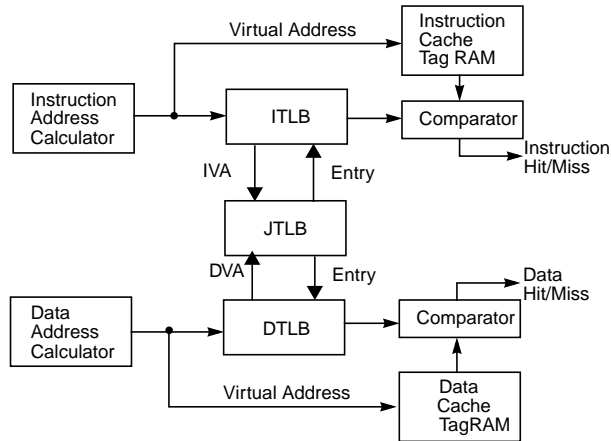
Figure 3 Address Translation During a Cache Access.
