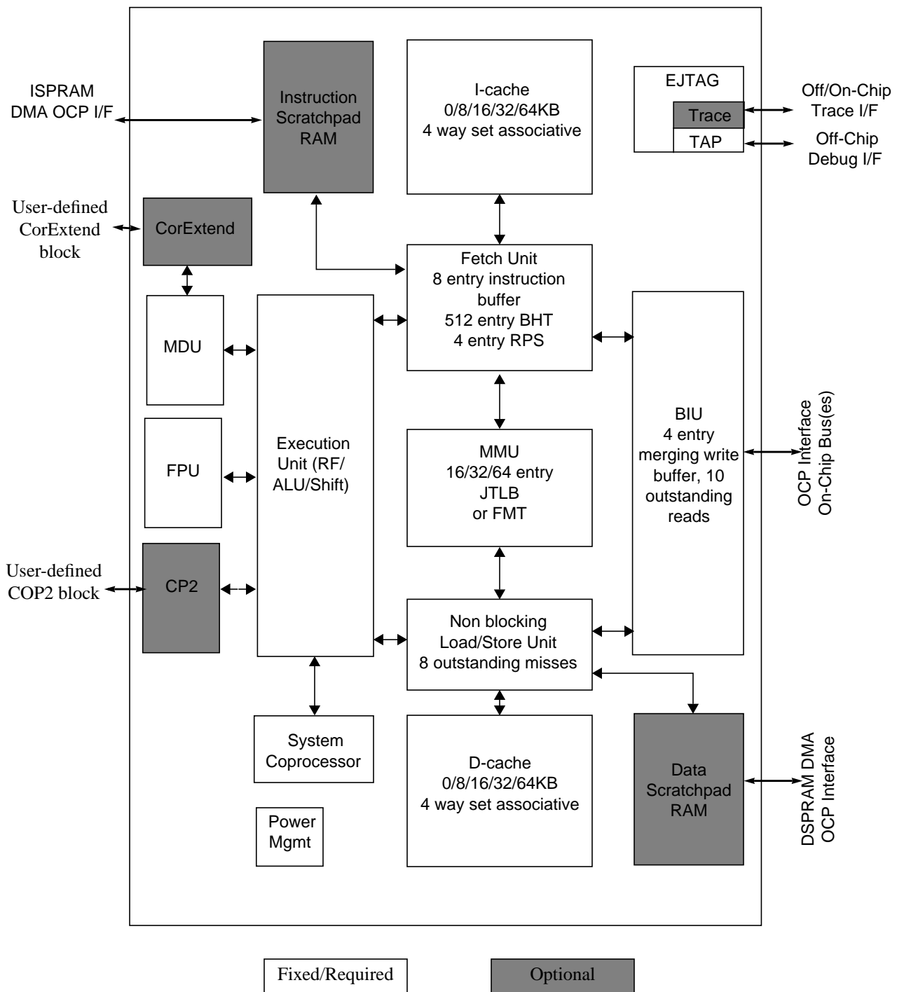
Figure 1 24Kf™ Core Block Diagram
