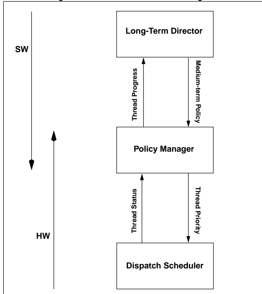
Figure 1 Thread Scheduler Block Diagram
