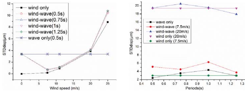
a. STD displacement versus wind speed
