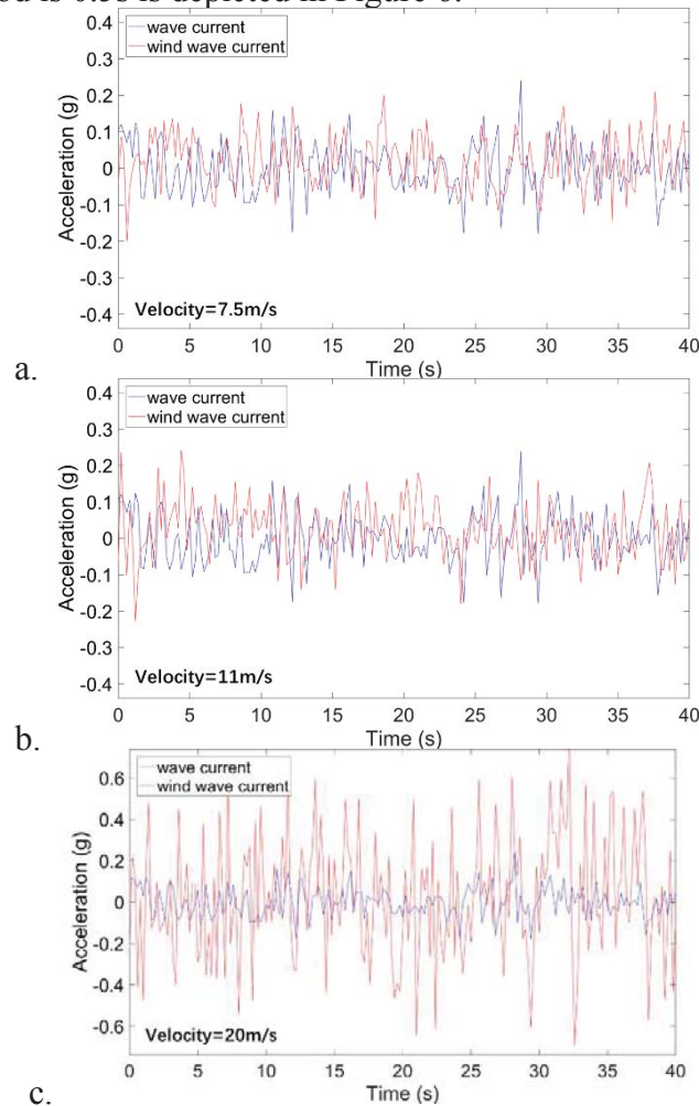
Figure 6 Accelerations of the tower model under wind-wave-current and wave-current loading states
