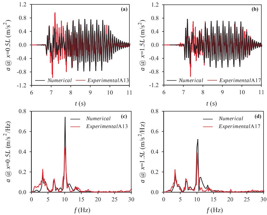
Figure 13: (a)-(b) Time history and (c)-(d) frequency content of the acceleration response at sensors 13 and 17 induced by Alaria Talgo VI train. Numerical prediction (black trace) vs. experimental measurements (red trace). Southbound train (track #1).
