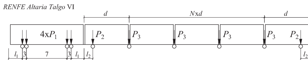
Figure 11: Renfe medium distance Altaria Talgo VI train axle scheme.
