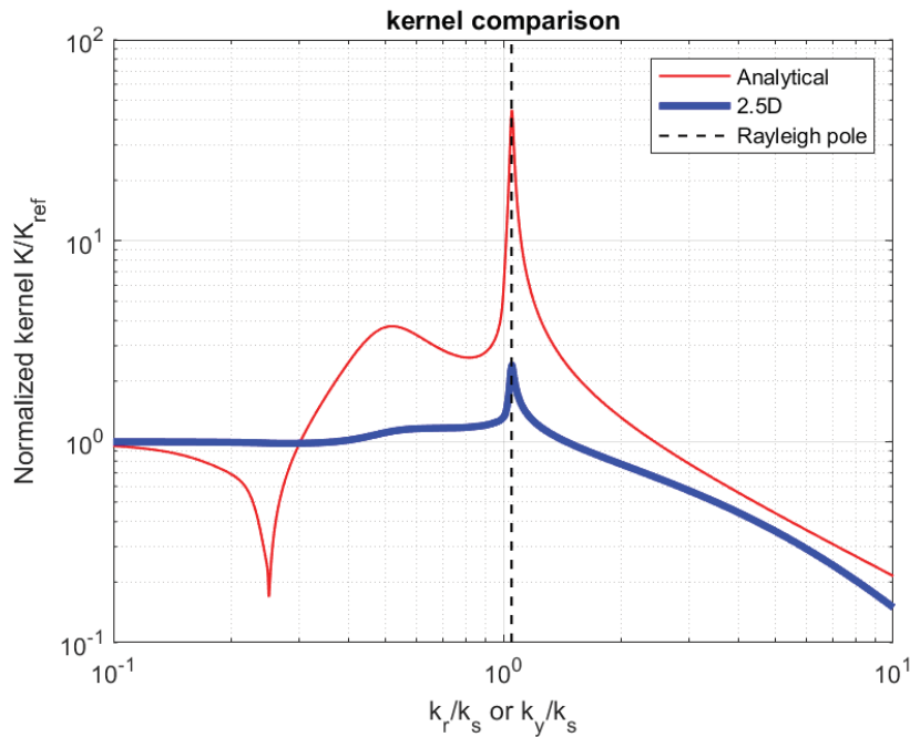
Figure 1. Comparison of two kernels calculated by means of analytical and 2.5D solutions, normalized with respect to the reference kernel calculated at the zero wavenumber. Note that the x-axis is the normalized wavenumber with respect to the shear wavenumber k_s ; and k_r and k_y are the radial- and y-direction wavenumbers, respectively, used in the analytical and 2.5D FE solutions.
