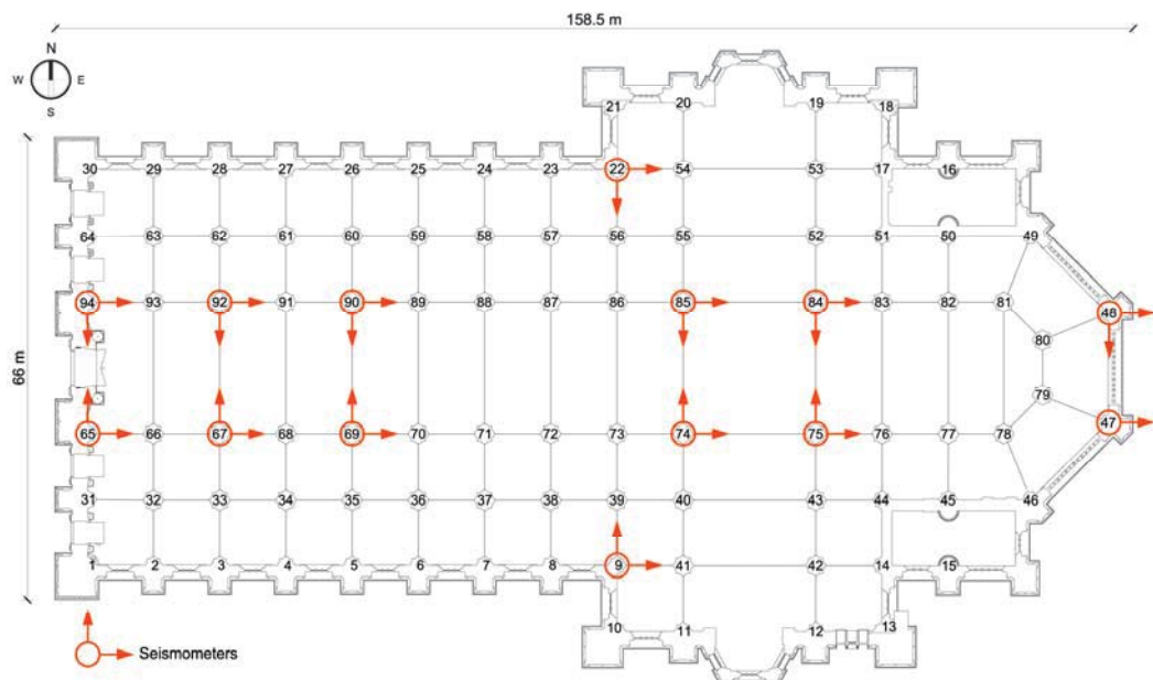
Figure 4: Plan of the Milan Cathedral (dimensions in m) and layout of the seismometers installed in the church.
