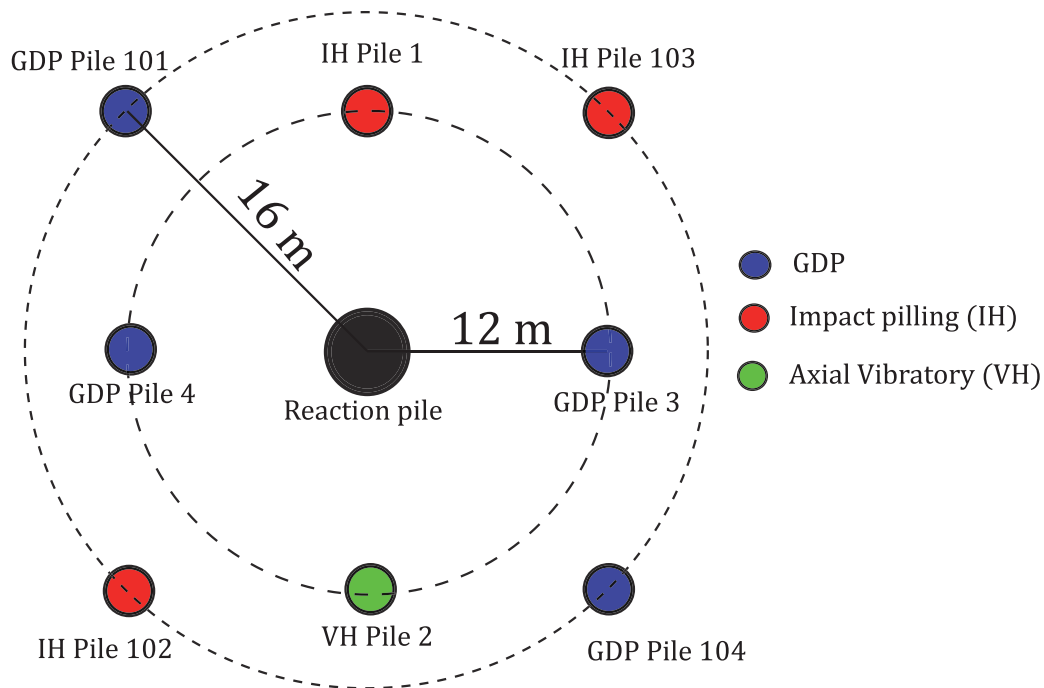
Figure 1: Pile layout
