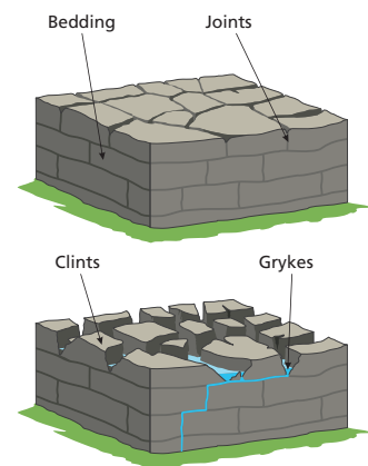
Limestone landscape, before and after carbonation.
