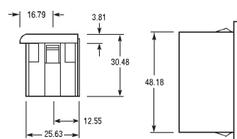
end frame
