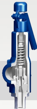
REYCO® RL14 ASME VIII, Threaded
