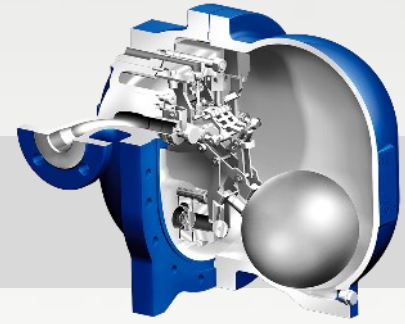
CONA®-P Pump trap
