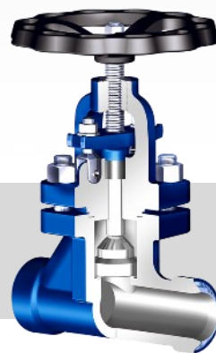
STOBU® Gland seal stop valves
