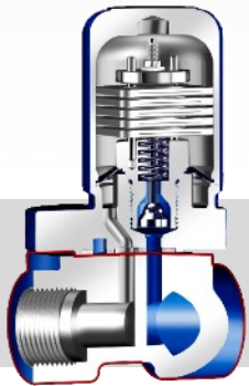
CONA® Universal Steam trap with flanges
