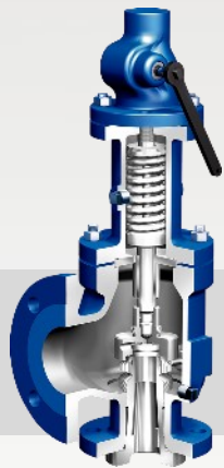
REYCO® R ASME VIII, API526 Full Nozzle
