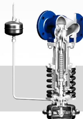
PREDEX® Excess pressure regulating valves
