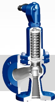
SAFE-P Standard safety valve
