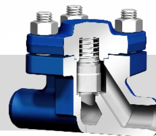
CHECKO®-D / V Check valves
