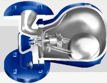
CONA-S Ball float
