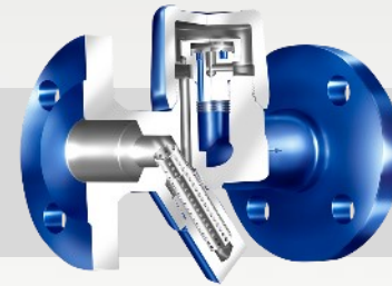
CONA®-TD Thermodynamic
