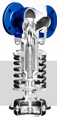
PREDU® Pressure reducing valves
