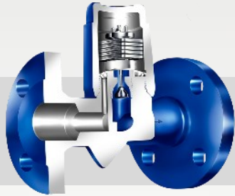
CONA®-B Bimetallic
