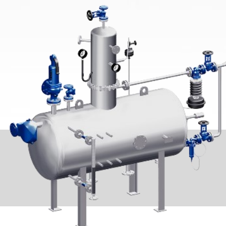
Feedwater Tank with deaerator dome
