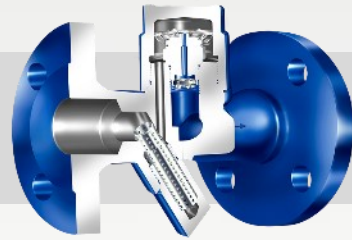
CONA®-M Thermostatic
