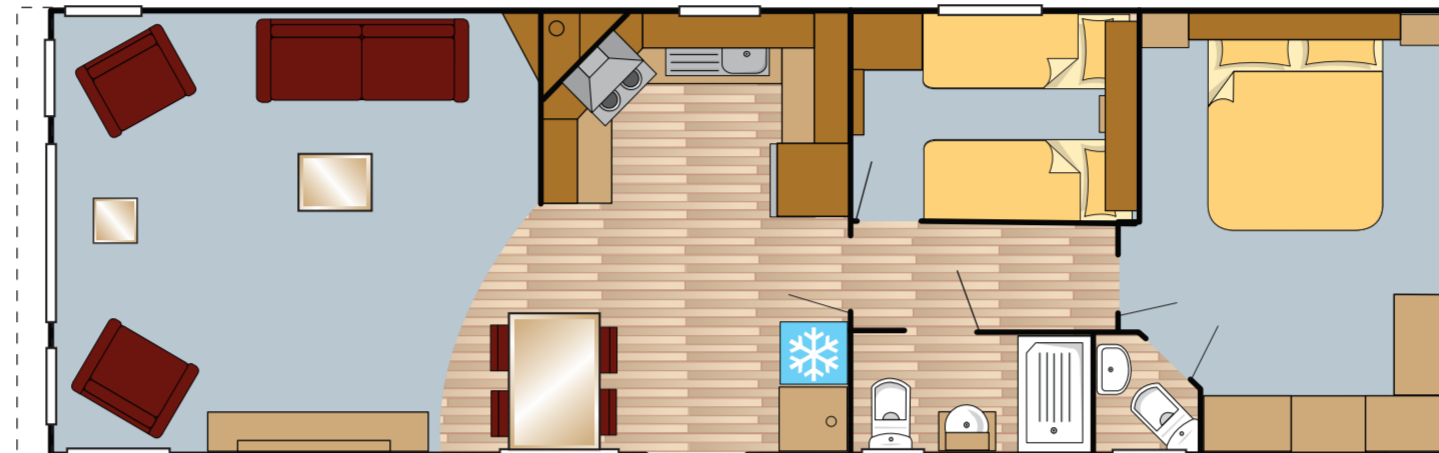
40x13 2 Bed
