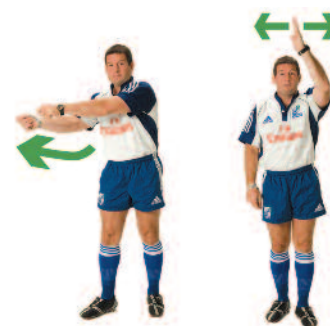
Forward pass
