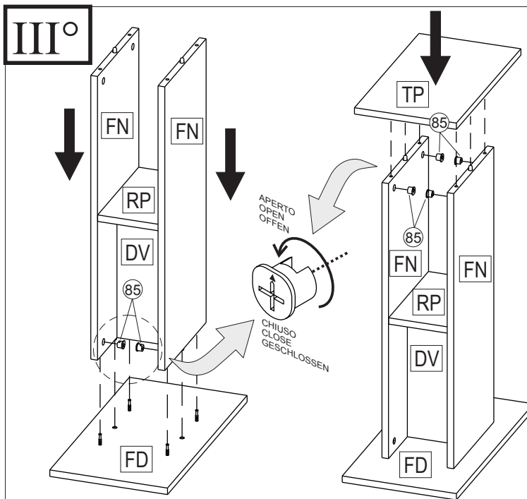
STAND 50 520x280x730
