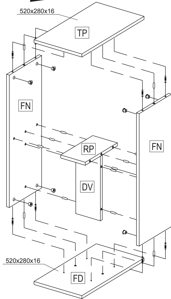
STAND 50 520x280x730
