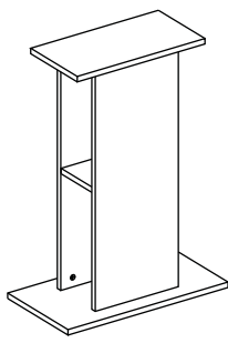
STAND 50 520x280x730
