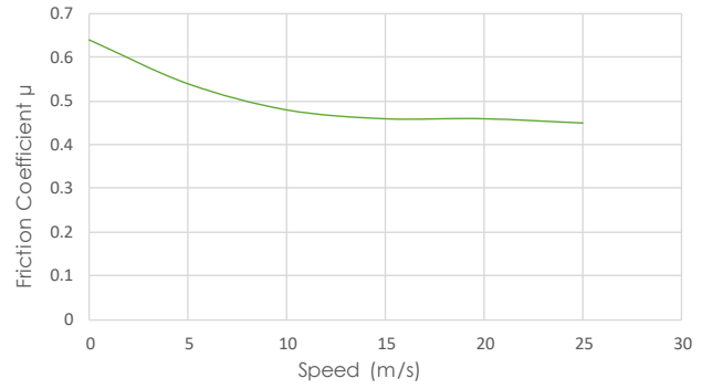
Speed Sensitivity
