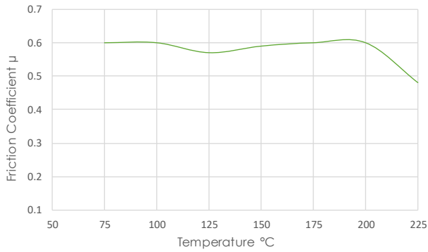
Temperature Sensitivity
