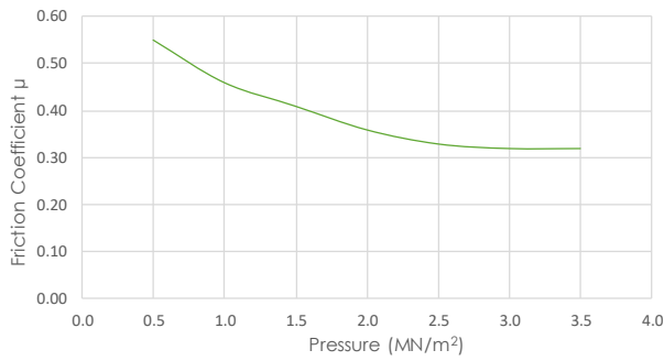
Pressure Sensitivity
