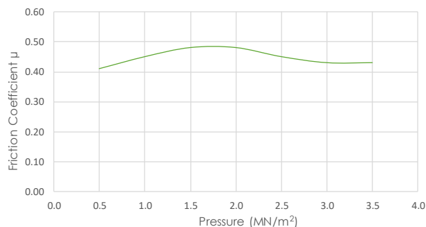
Pressure Sensitivity
