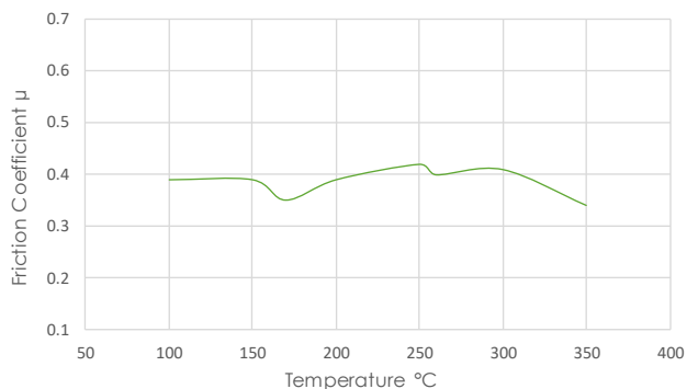
Temperature Sensitivity
